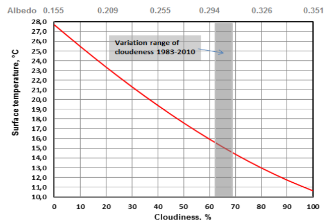
FIG. 3. THE SURFACE TEMPERATURE AS A FUNCTION OF CLOUDINESS ACCORDING TO THE ENERGY BALANCE EQUATIONS (2)...(6).
