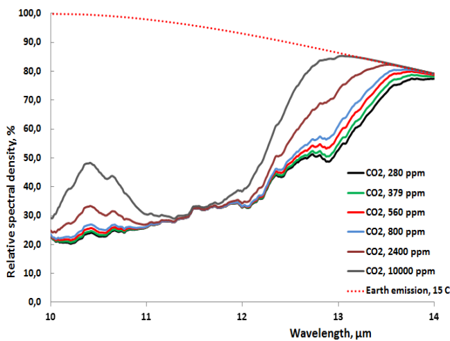
FIG. 2. THE TOTAL ABSORPTION BAND GRAPHS FOR INCREASED CO 2 CONCENTRATIONS IN THE AGA 2012 CONDITIONS IN THE TROPOSPHERE.
