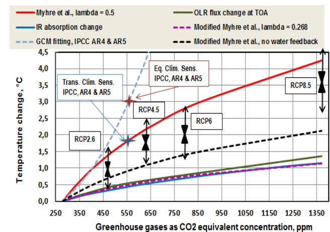
FIG. 4. GLOBAL WARMING INCREASE ACCORDING TO DIFFERENT SIMULATION AND ESTIMATION METHODS.
