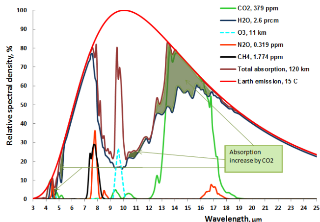
FIG 1. THE ABSORPTION BAND GRAPHS OF GH GASES IN THE ATMOSPHERE IN THE AGA CONDITIONS 2005. THE GREEN-SHADED AREAS INDICATE A TOTAL GH IMPACT OF CO 2 CONCENTRATION OF 379 PPM.
