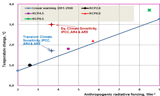
FIG. 5. THE GLOBAL WARMING VALUES ACCORDING TO THE ANTHROPOGENIC RADIATIVE FORCING BY IPCC.
