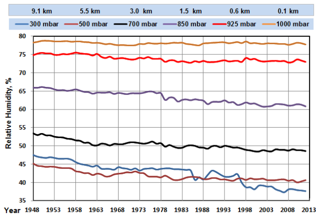
FIG. 6. RELATIVE HUMIDITY TRENDS ACCORDING TO NOAA AT DIFFERENT ALTITUDES IN THE TROPOSPHERE.
